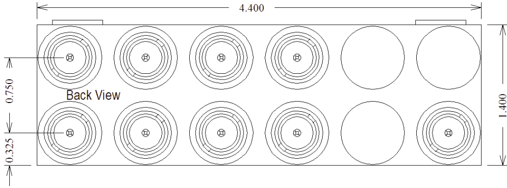
Figure 7: input / output connectors
